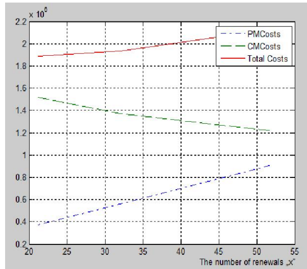
Fig. 7. The variation of costs with power line maintenance depending by the optimal number of renewals
