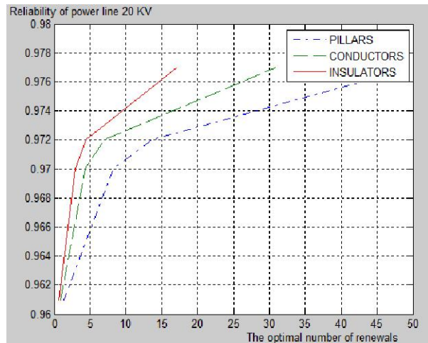
Fig. 8. The variation of renewals number on the electrical power line components, depending by minimum reliability required on each component
