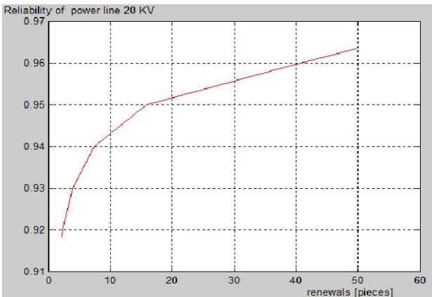
Fig. 5. The variation of the optimal number of renewals with minimum reliability required line
