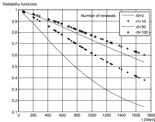
Fig. 1. Influence of the number of renewals on system reliability
