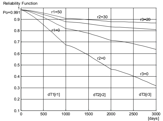
Fig. 3. Influence of the renewals “ r_i ” on the reliability of the line, for three intervals of time \Delta T_i
