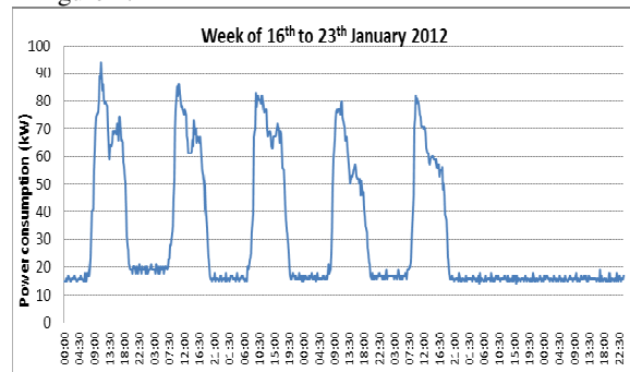
Fig. 2 - Electrical Load profile of the building – Mid-winter
