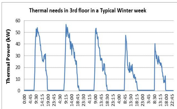
Fig. 3 - Thermal Load profile of the 3 rd floor - winter
