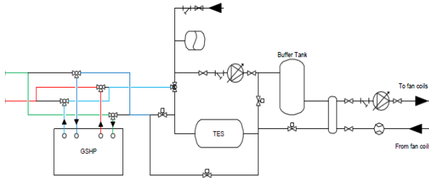
Fig. 9 - Internal hydraulic loop with the storage tank.
