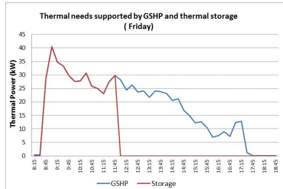
Fig. 5 - 100kWh storage capacity supports thermal needs during 3,5h
