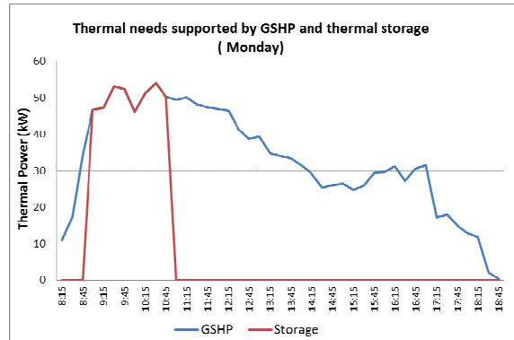
Fig. 4 - Capacity Storage of 100kwh supports thermal needs during 2h
