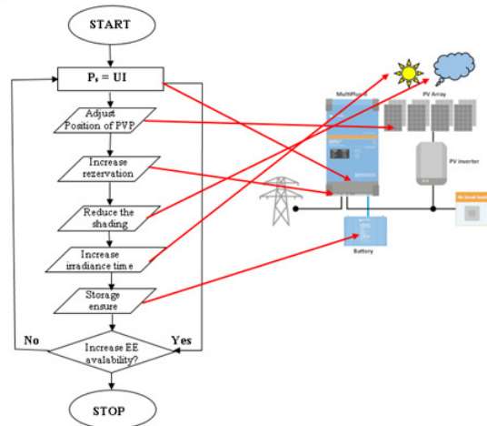
Fig. 4 - Logic diagram for fuzzy controllers and regulators of photovoltaic panels
