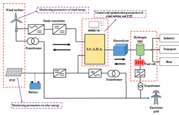
Fig. 1 - Structure of an intelligent hybrid RES-Hydrogen plants
