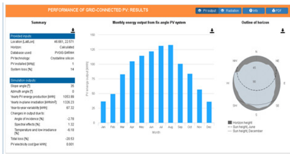
Fig. 3 - Monthly solar radiation and energy output from PV system
